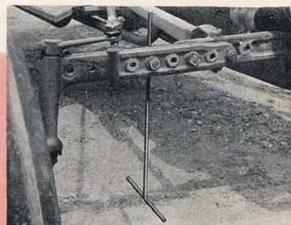
STEERING POINTER
